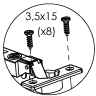
DETAIL L
