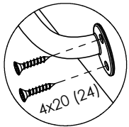
DETAIL J
