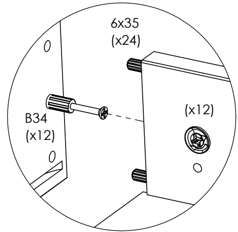
DETAIL H
